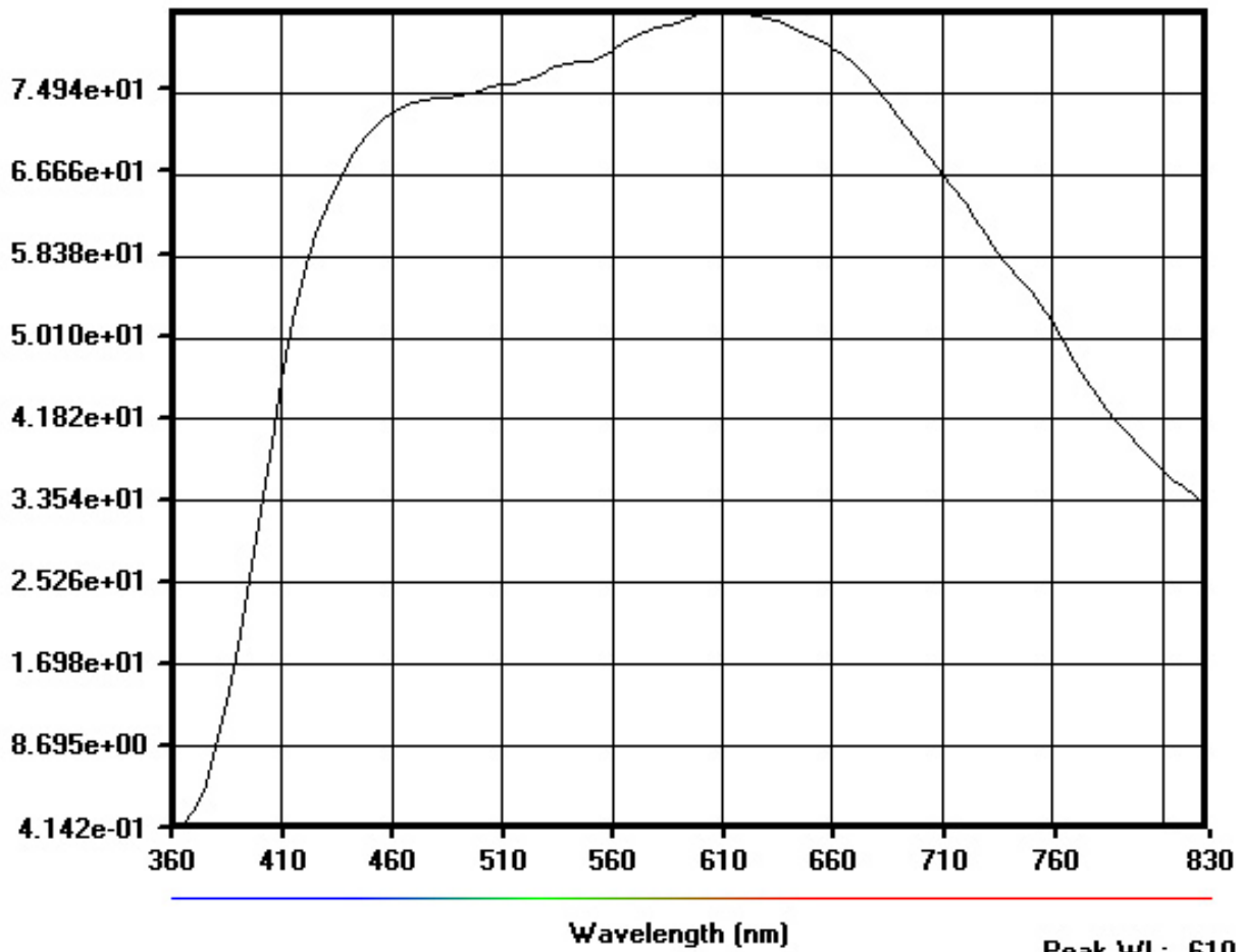
BUSHNELL LEGEND 8X42MM LEFT TRANSMITTANCE FINAL 01/06/06
