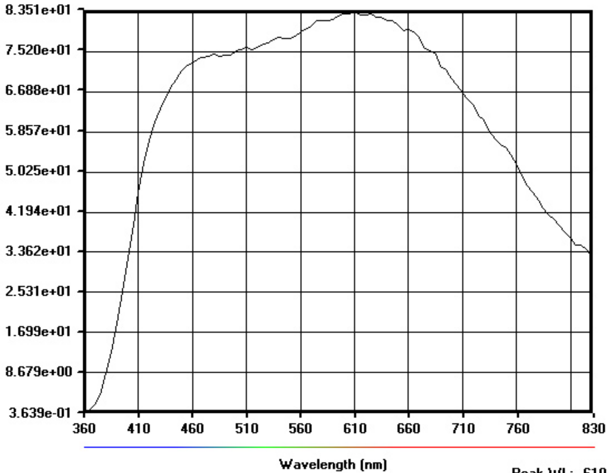
BUSHNELL LEGEND 8X42MM RIGHT TRANSMITTANCE FINAL 01/06/06
