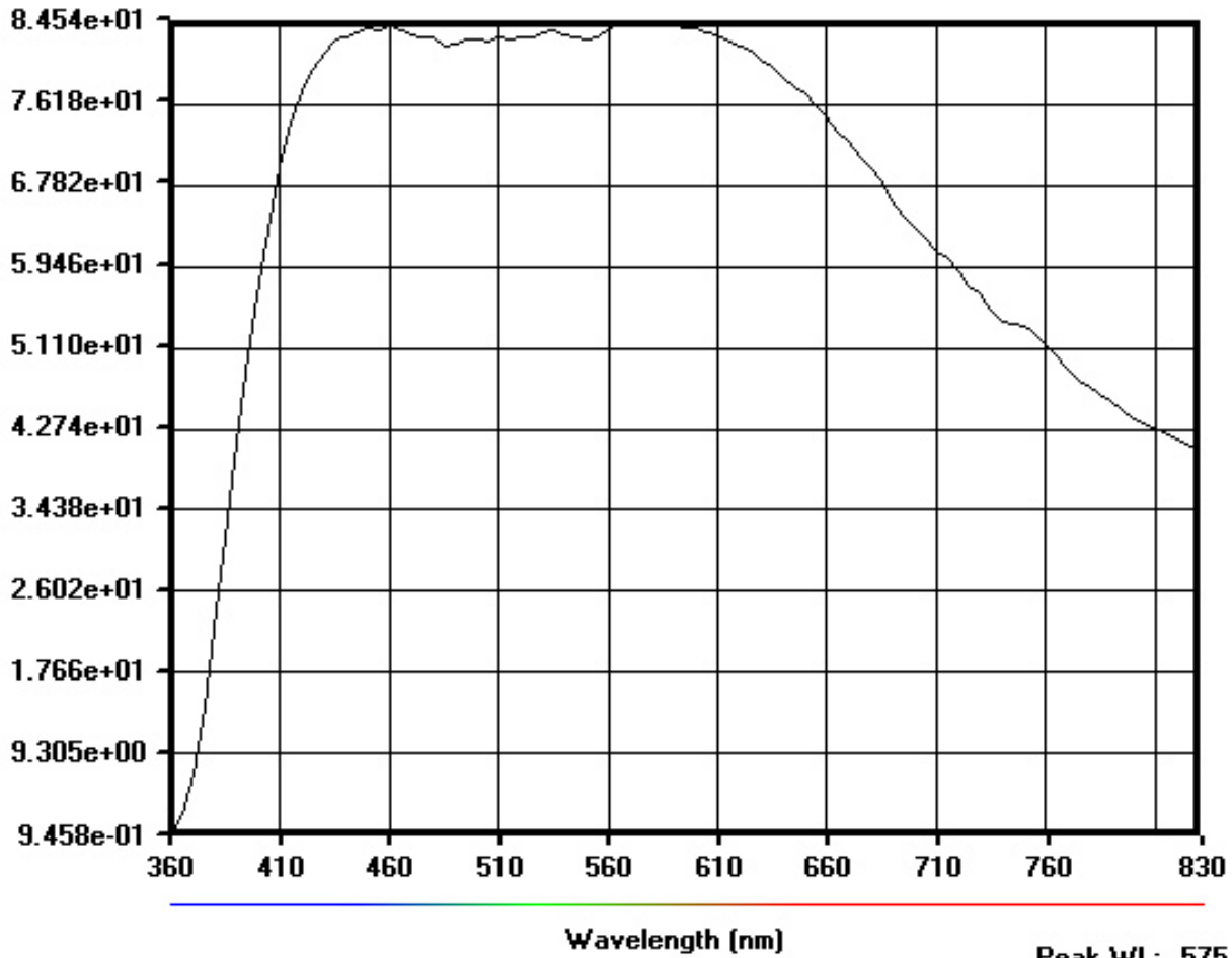
PENTAX DCF HR II 8X42MM LEFT TRANSMITTANCE FINAL 01/06/06
