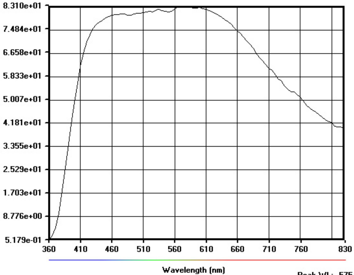
PENTAX DCF HR II 8X42MM RIGHT TRANSMITTANCE FINAL 01/06/06
